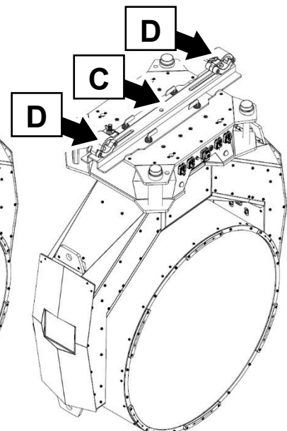
Installation with one Truss Mount Bar
