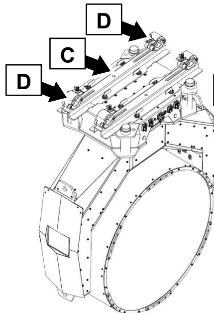
Installation with two Truss Mount Bars
